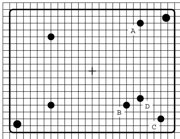
Bottom View (Grid Spacing 0.1")
